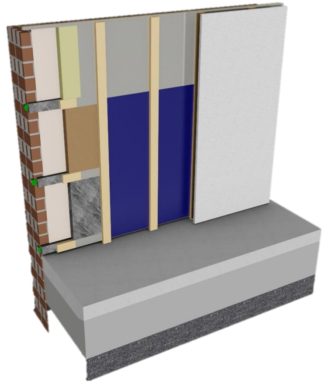
Vertical Battens
